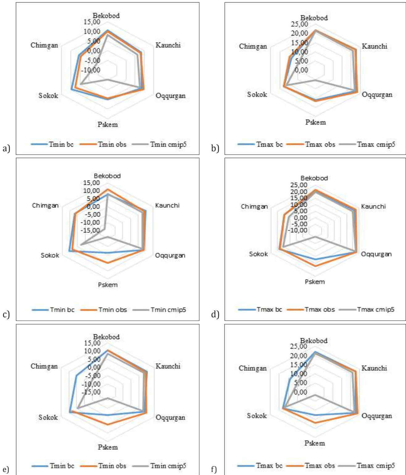
Figure 3. Observed, CMIP5 and bias-corrected temperature: a) Annual minimum temperature of 2000 b) Annual maximum temperature of 2000 c) Annual minimum temperature of 2010 d) Annual maximum temperature of 2010 e) Annual minimum temperature of 2018 f) Annual maximum temperature of 2018
