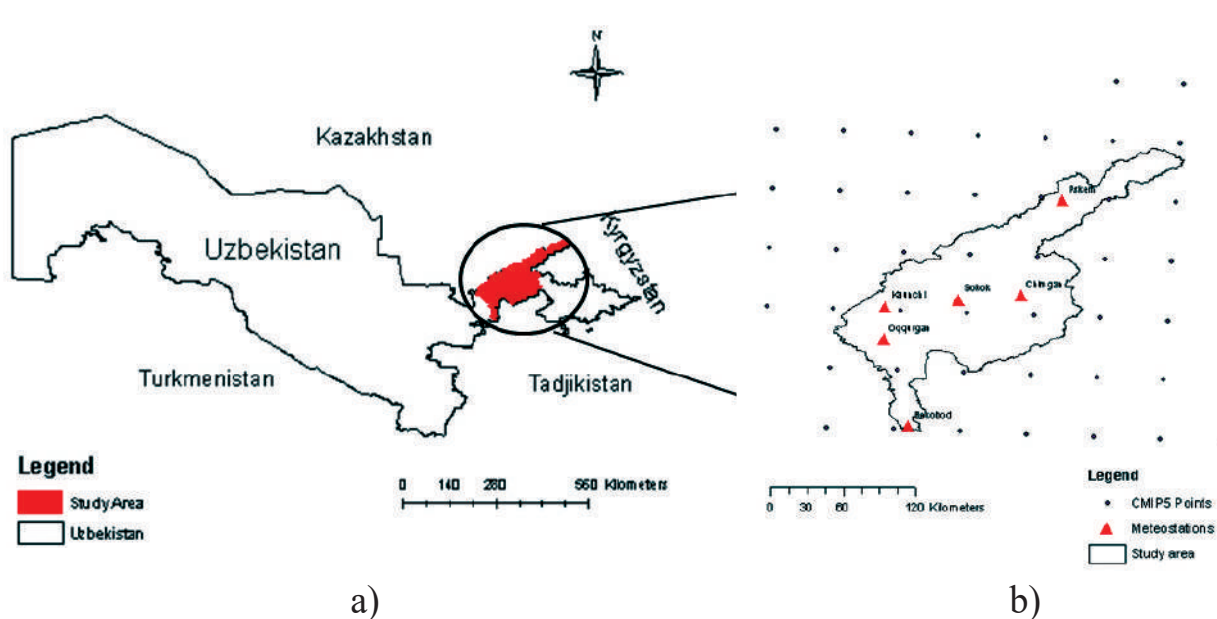
Figure 1. Overview of the study area a) geographical location b) CMIP5 grid boxes and bias-corrected meteorological stations
